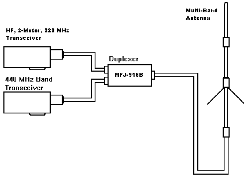
Connection Diagram 1
