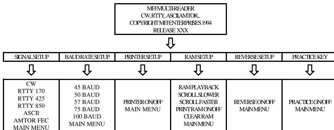
MFJ-462B MultiReader™ Menu Layout
