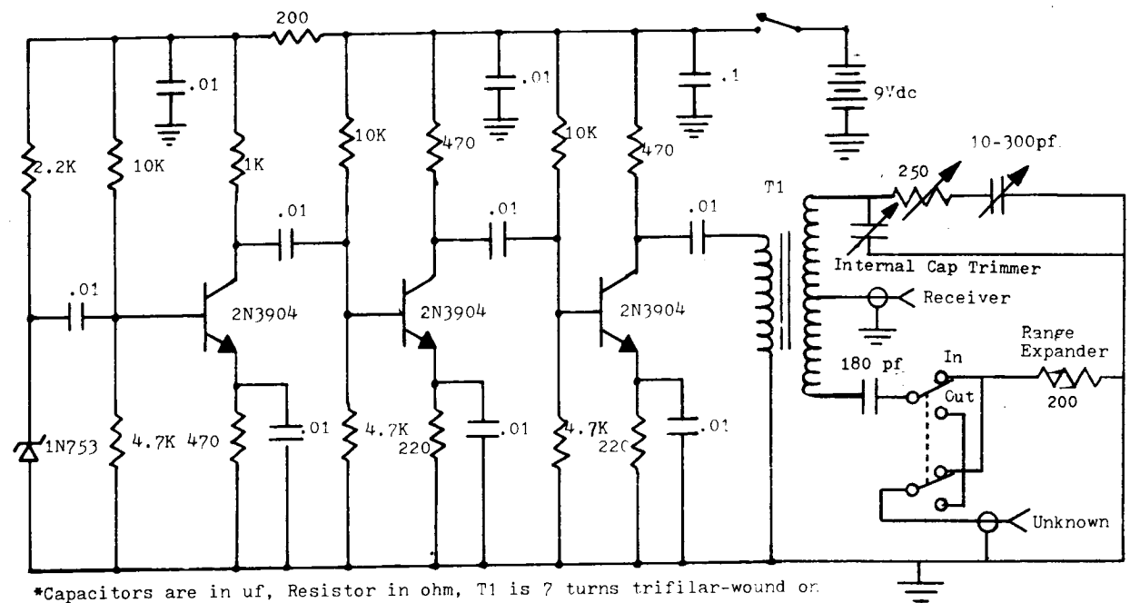
MFJ-202B RF Noise Bridge Circuit Diagram
